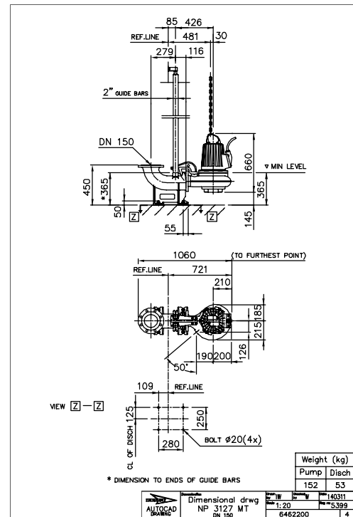
Figure 74: MT, P-installation
