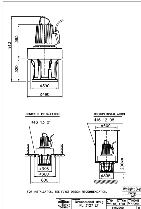
Figure 106: LT, L-installation
