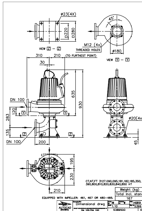
Figure 27: HT, T-installation
