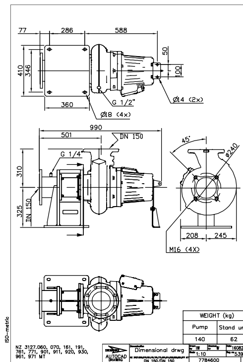
Figure 87: MT, Z-installation
