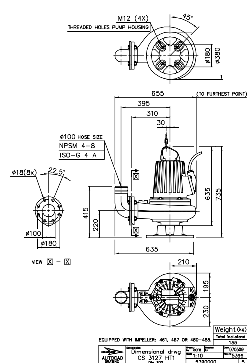
Figure 24: HT, S-installation
