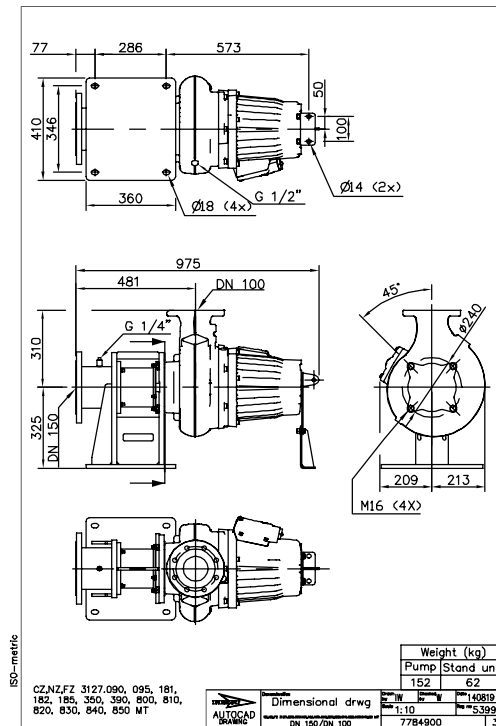
Figure 88: MT, Z-installation
