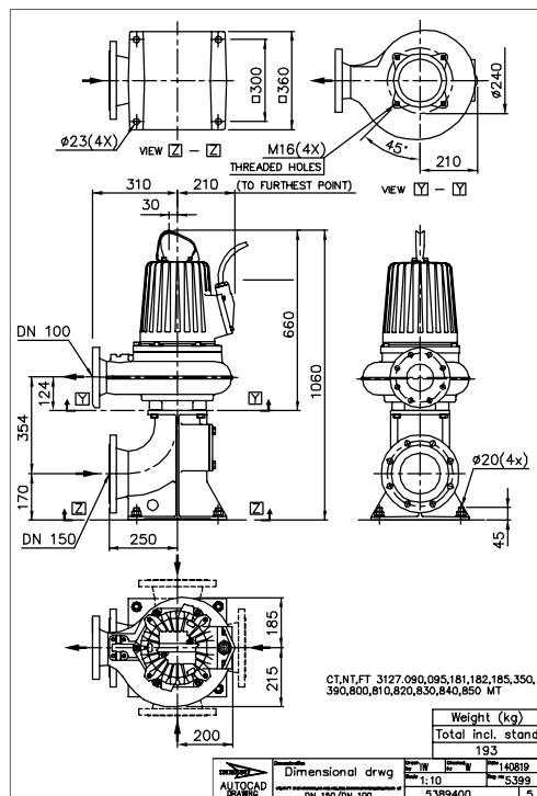
Figure 84: MT, T-installation
