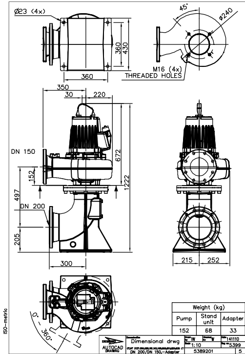
Figure 70: LT, T-installation
