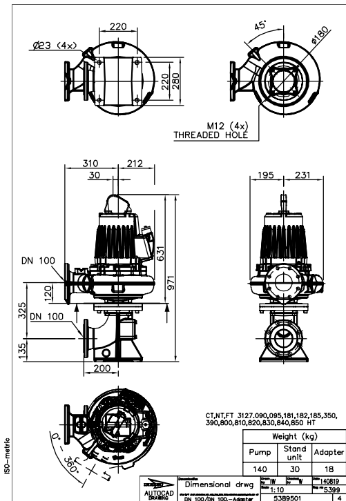
Figure 28: HT, T-installation
