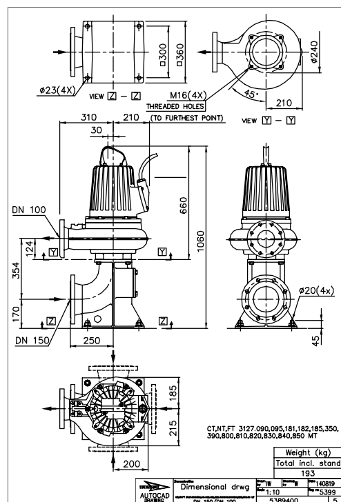
Figure 16: MT, T-installation
