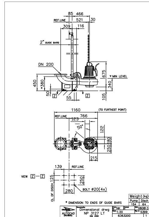
Figure 61: LT, P-installation
