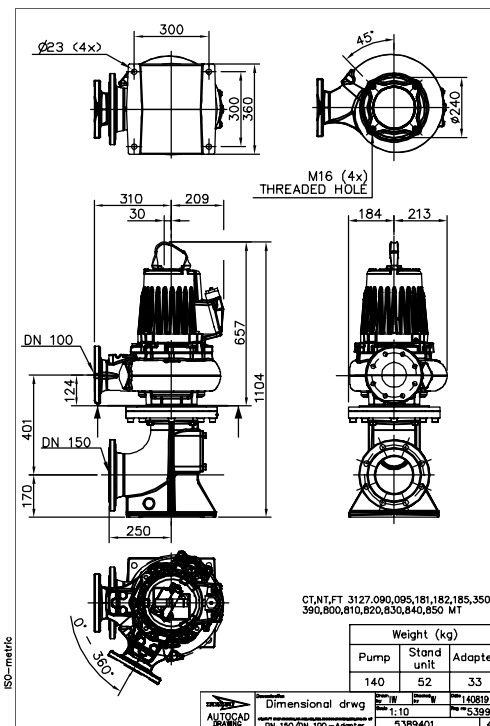
Figure 85: MT, T-installation
