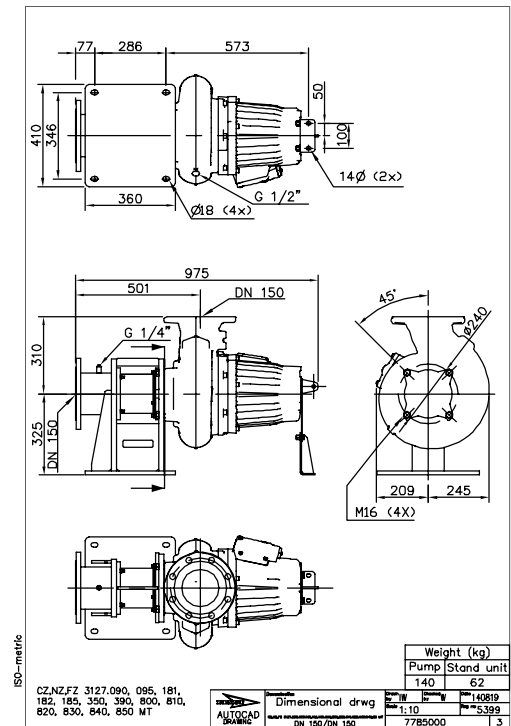
Figure 89: MT, Z-installation
