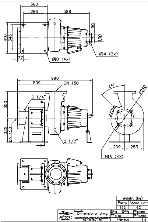
Figure 72: LT, Z-installation
