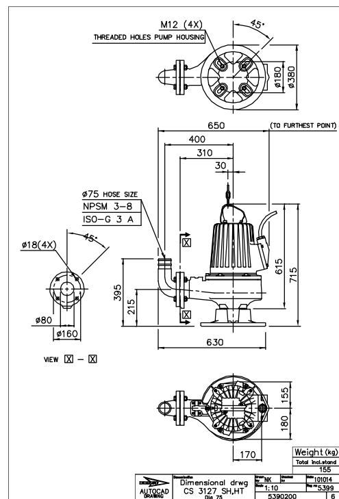
Figure 26: HT/SH, S-installation
