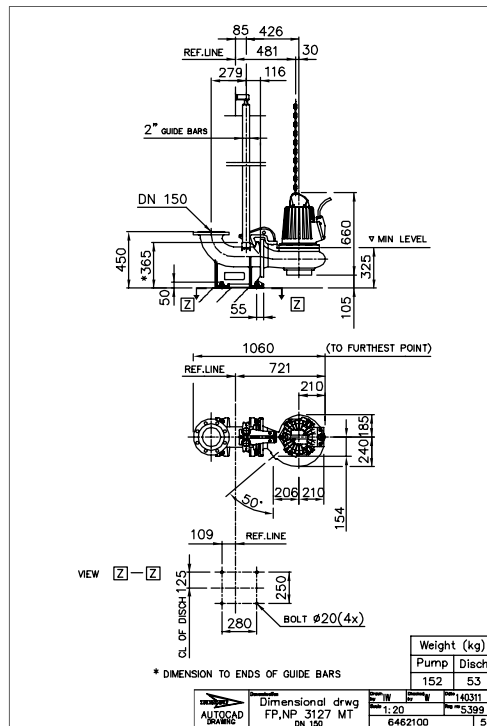
Figure 73: MT, P-installation
