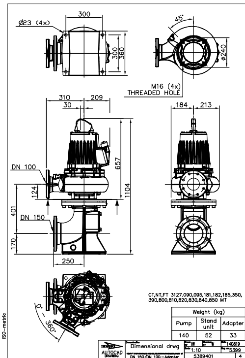
Figure 47: MT, T-installation
