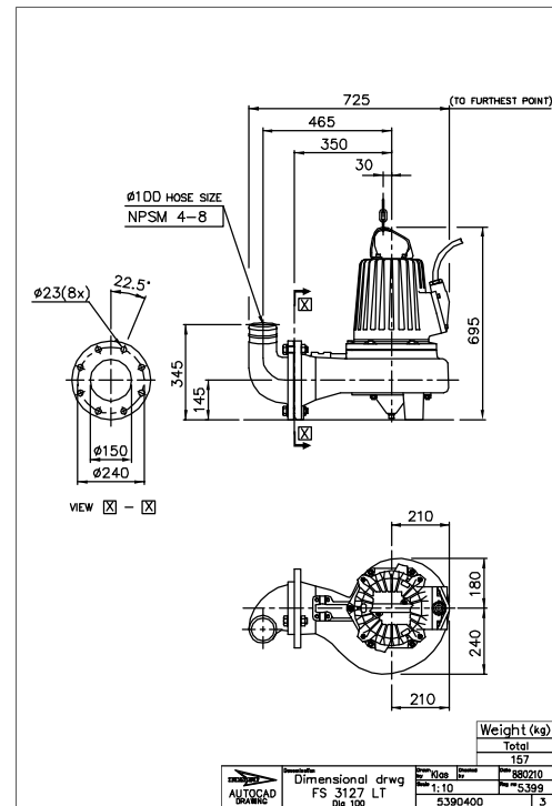
Figure 38: LT, S-installation
