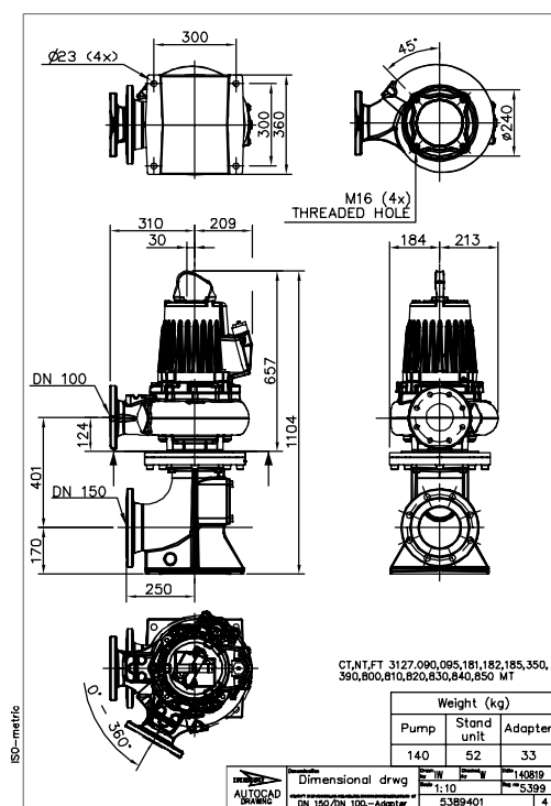
Figure 17: MT, T-installation
