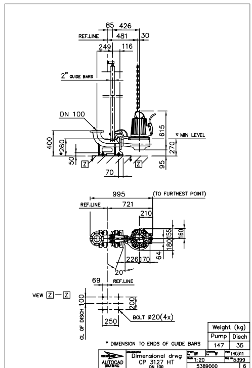
Figure 22: HT, P-installation
