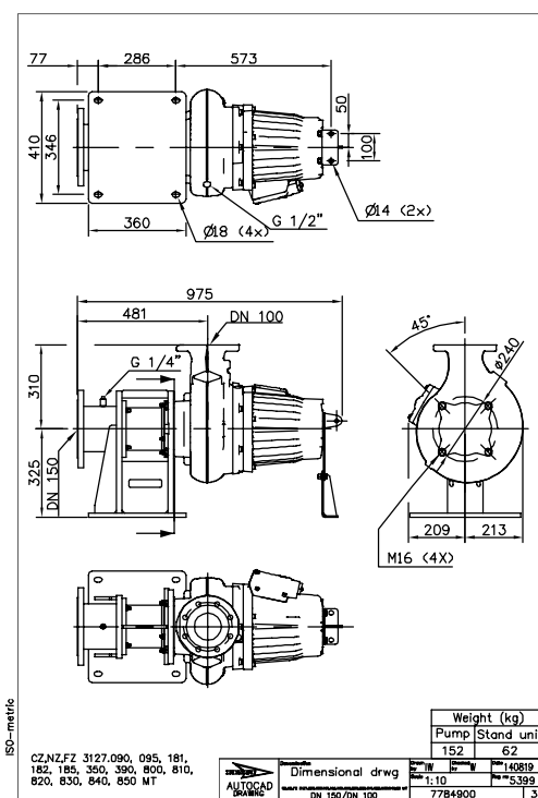
Figure 18: MT, Z-installation
