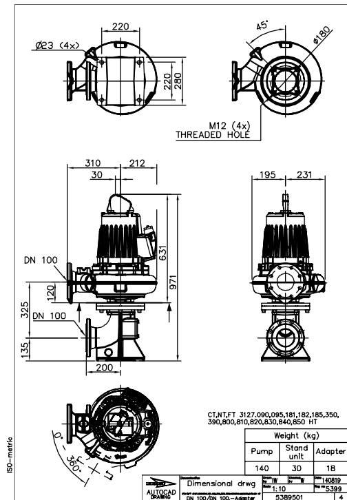
Figure 53: HT, T-installation
