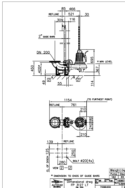
Figure 37: LT, P-installation
