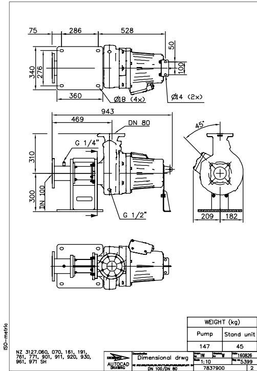
Figure 105: SH, Z-installation
