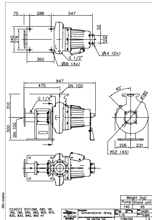
Figure 30: HT, Z-installation
