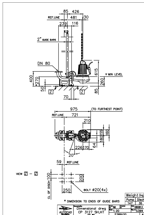
Figure 23: HT/SH, P-installation
