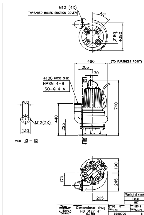
Figure 57: HT, S-installation
