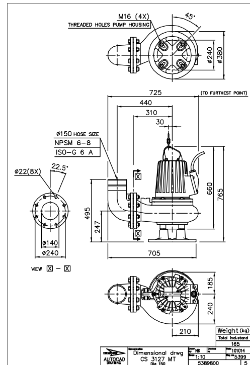
Figure 12: MT, S-installation
