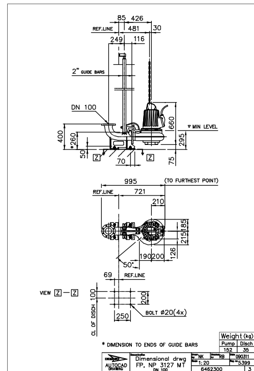
Figure 40: MT, P-installation
