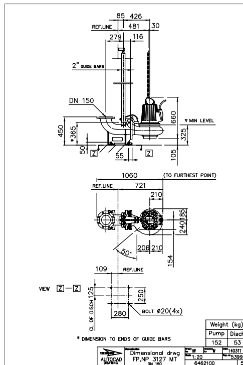
Figure 39: MT, P-installation
