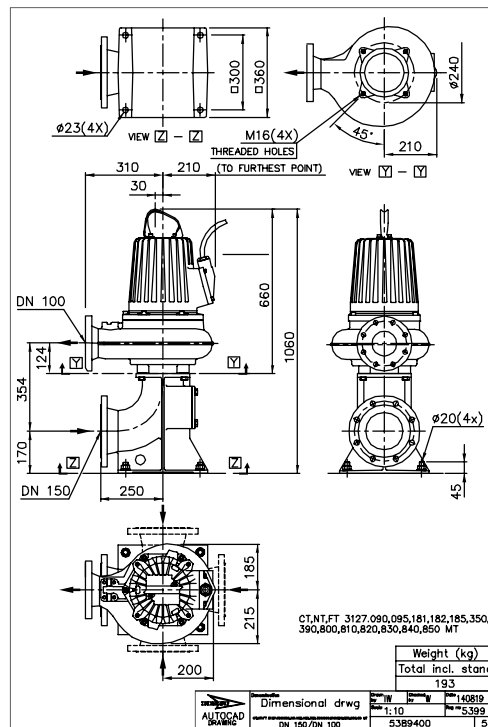
Figure 46: MT, T-installation
