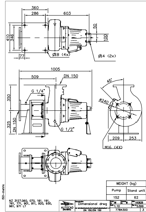
Figure 71: LT, Z-installation
