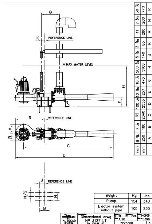
Figure 63: LT, P-installation
