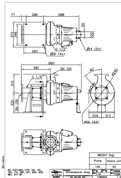
Figure 86: MT, Z-installation
