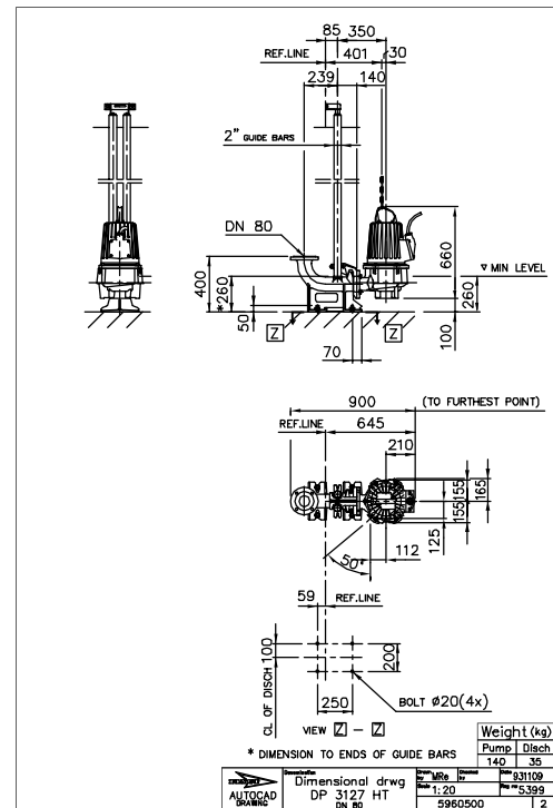
Figure 34: HT, P-installation
