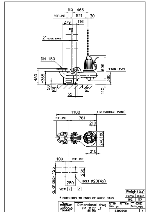
Figure 36: LT, P-installation
