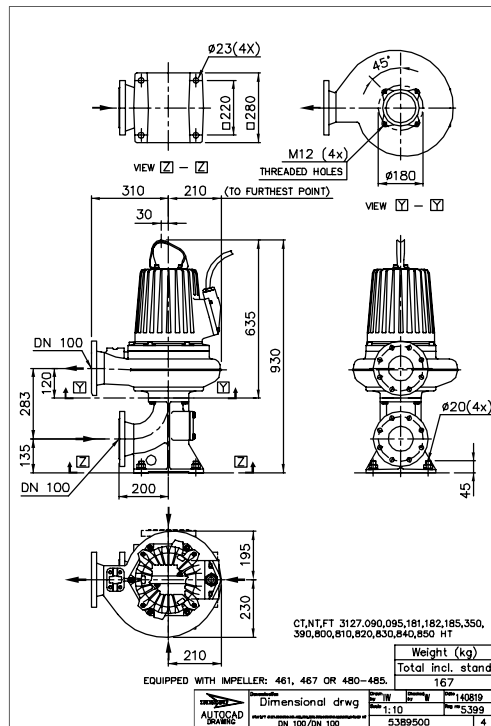
Figure 52: HT, T-installation
