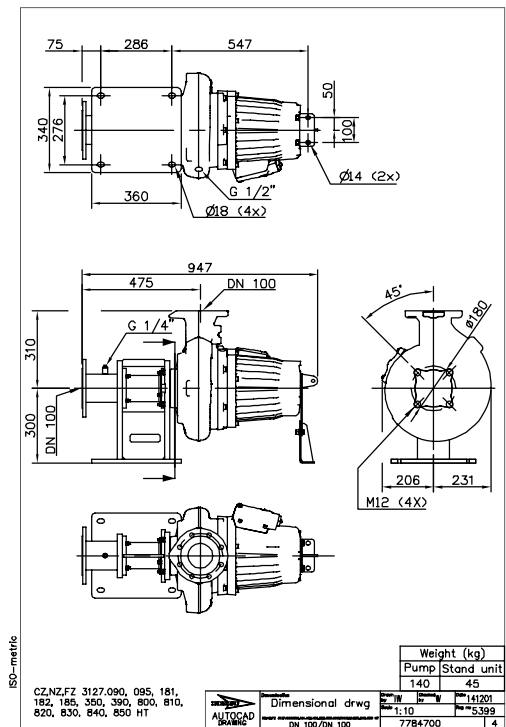
Figure 97: HT, Z-installation
