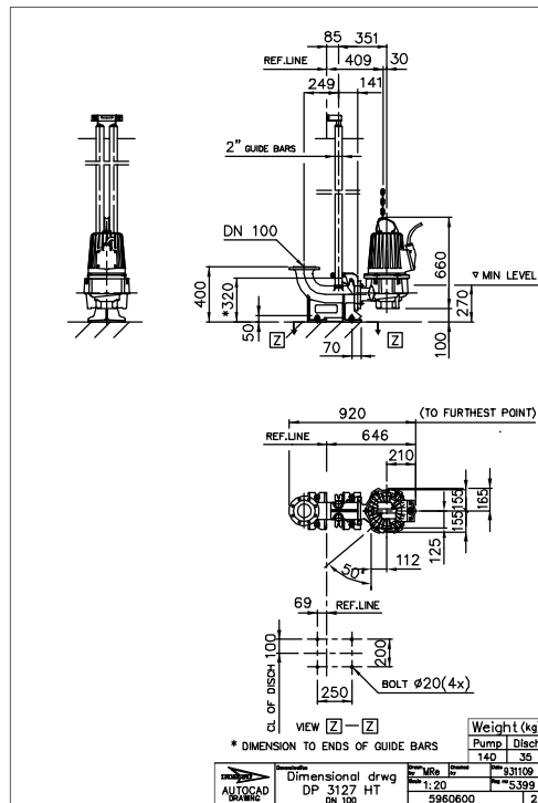
Figure 33: HT, P-installation
